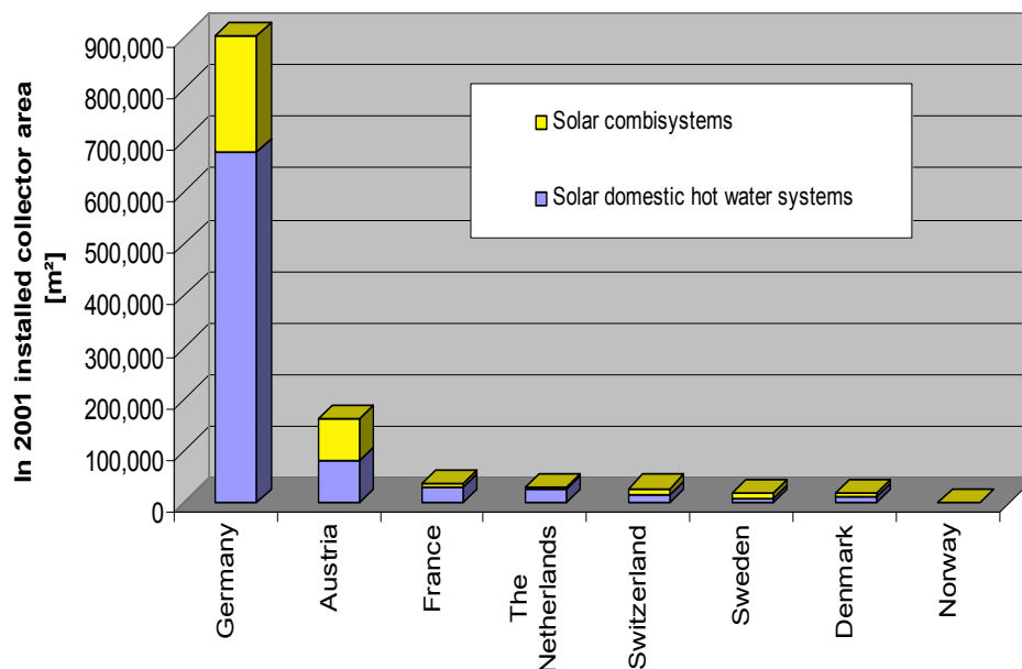
Figure 2. Installed collector area in different European countries. The yellow parts represent the collectors for combisystems. The figure is from Weiss [23].
