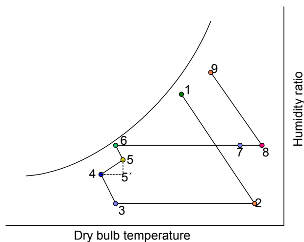
Fig. 3.4.2 Desiccant cooling process
