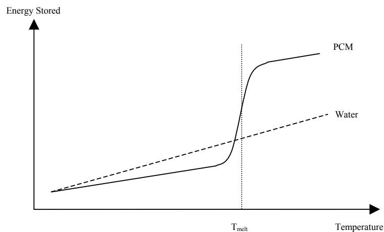
Figure 15. Comparison of PCM and Water based storage
