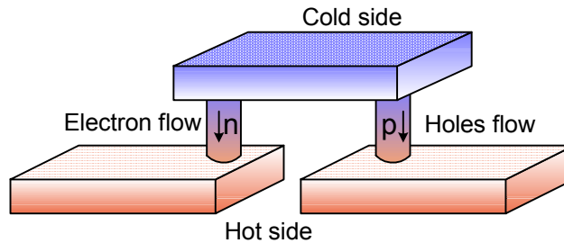
Fig. 3.8.1 Peltier's element
