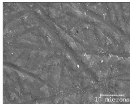
Fig-9 SEM photograph of a typical grinded surface 2000 X
