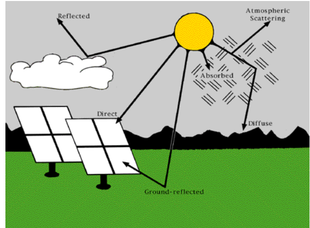
Figure 2: Sketches of the solar radiation through the atmosphere. (From http://www.volker-quaschnig.de/fotos/messung/index_e.html and http://rredc.nrel.gov/solar/pubs/shining/page12_fig.html )
