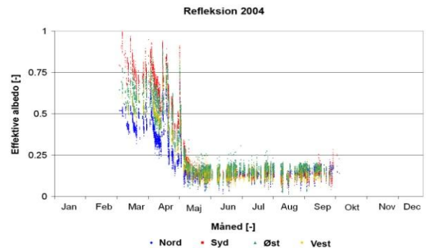
Fig. 2: The Effective albedo 2004.
