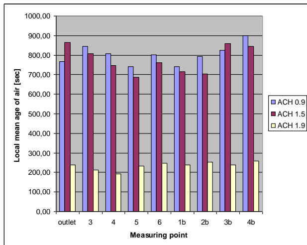
Figure 4. Local mean age of air at different measuring points in the test room.
