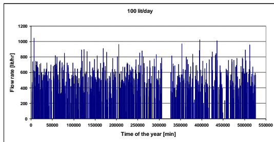
Fig. 2. Task 26 DHW profile during the whole year.
