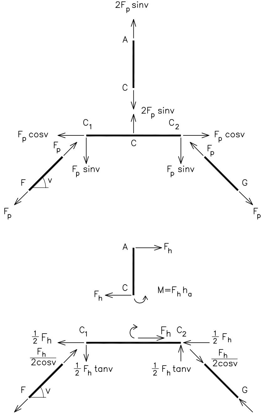
Figure 3. Section forces in damping system.
