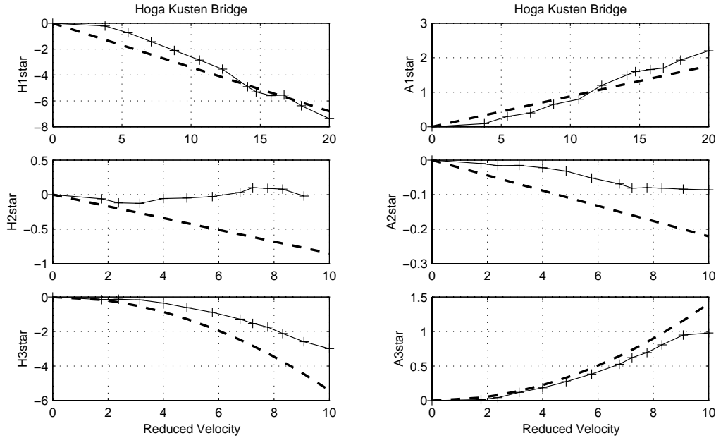
Figure 4: Variations of H^*_{1,2,3} and A^*_{1,2,3} with reduced velocity for the Högä Kusten Bridge. The dashed lines are predictions derived from quasi-steady aerodynamics using the coefficients of Fig. 2 and n = 0.25 .
