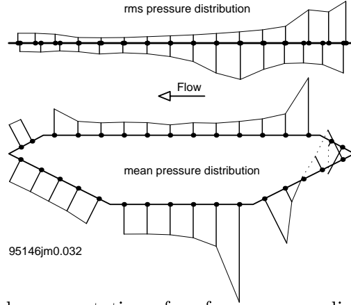
Figure 5: Vector field representation of surface pressure distribution on B/D=5 , medium spire exposure, with railings, 15 \text{ ms}^{-1} . Scaling: depth of deck= mean C_p of 1 and rms C_p of 0.5. Polarity: negative away from the surface. The rms distribution is given for the projected tributary area.
