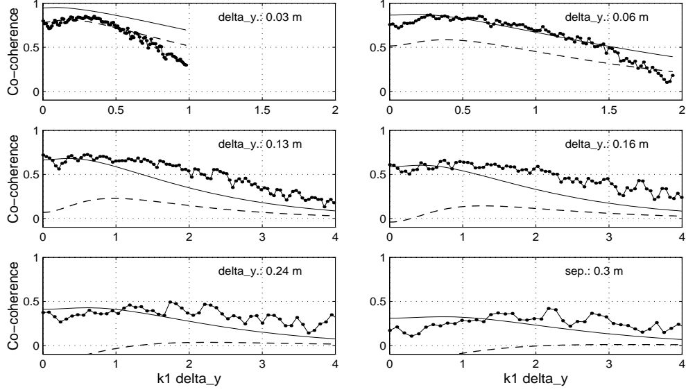
Figure 26: Co-coherence as a function of k_1 \Delta y for the lift forces (dotted line) for B/D = 5 and for the wind for the grid exposure . Solid line: v with L_{coh} = 0.18 and \mathcal{L} = 0.085 \text{ m} ; dashed line: w with L_{coh} = 0.12 and \mathcal{L} = 0.09 \text{ m} .
