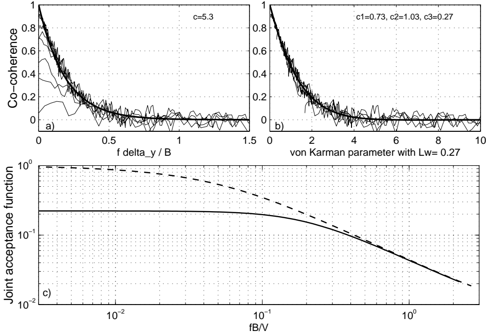
Figure 3: Variations of the joint acceptance function with reduced velocity for a uniform mode shape \mu(y) = 1 for two representations of the wind co-coherence: a) solid line: cocoh_w(\Delta y, f) = \exp[-cf\Delta y/B] ; b) solid line: cocoh_w(\Delta y, f) = \exp[-c_1\gamma^{c_2}] \cos(c_3\gamma) . On c) |J_z(f_j^*)|^2 was calculated using the fits based on f\Delta y/B (dashed line) and based on the von Kármán parameter (solid line).
