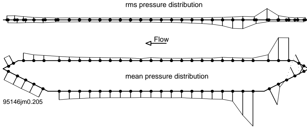
Figure 40: Surface pressure distribution on B/D=10 , smooth flow, without railings, 9 \text{ ms}^{-1} . Scaling: depth of deck= mean C_p of 1 and rms C_p of 0.5. Polarity: negative away from the surface. The rms distribution is given for the projected tributary area.
