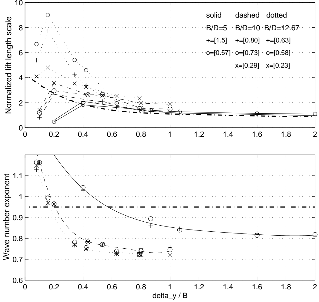
Figure 26: Results of the fit of the measured co-coherence of the lift forces as a function of \Delta y/B . The ordinate of the top graph is the lift length scale L_L obtained from the fit of equation (27) and normalized by the length scale L of the incident flow. The chain-dotted line refers to the theoretical calculations with the 3-D model. The wave number exponent refers to \mathbf{a} in k_1^{\mathbf{a}} .
