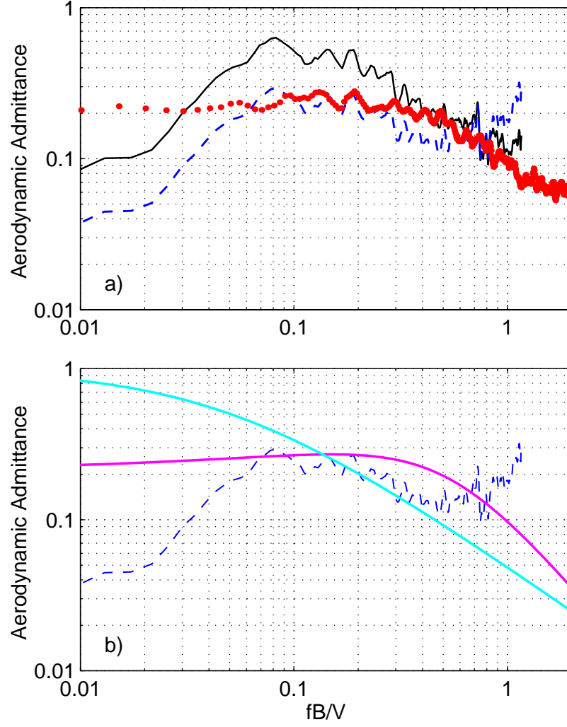
Figure 7: Variations of the pitching moment aerodynamic admittance as a function of fB/V . On a) , dots: admittance directly measured from a chord-wise strip as reported in Larose et al. (1997), for L_w/B=0.58 ; solid line: segmental admittance; dashed line: cross-sectional admittance determined with the present method. On b) , light solid line: Sears' function; dark solid line: empirical model of 2-D aerodynamic admittance of Larose & Mann (1998) for L_w/B=0.60 ; dashed line: cross-sectional admittance determined with the present method.
