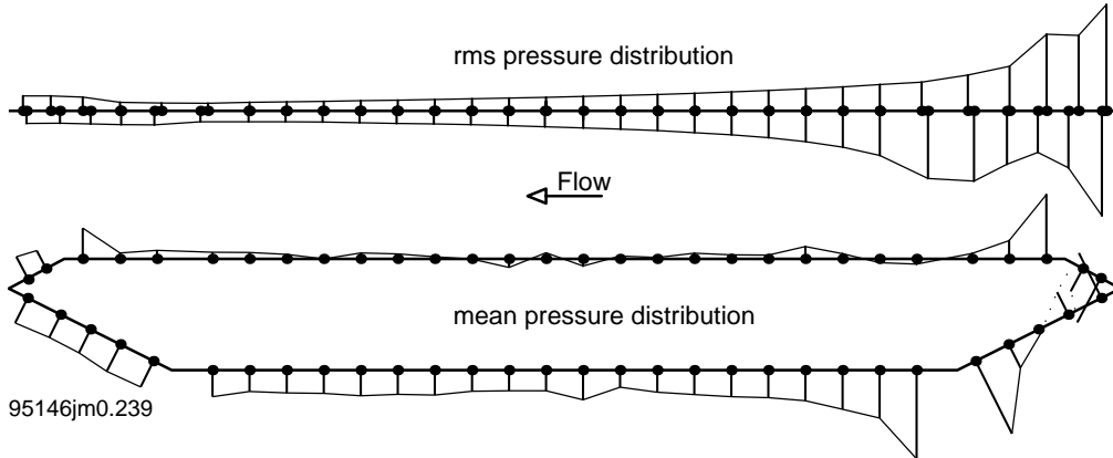
Figure 6: Vector field representation of surface pressure distribution on B/D=10 , large spire exposure, with railings, 15 \text{ ms}^{-1} . Scaling: depth of deck= mean C_p of 1 and rms C_p of 0.5. Polarity: negative away from the surface.
