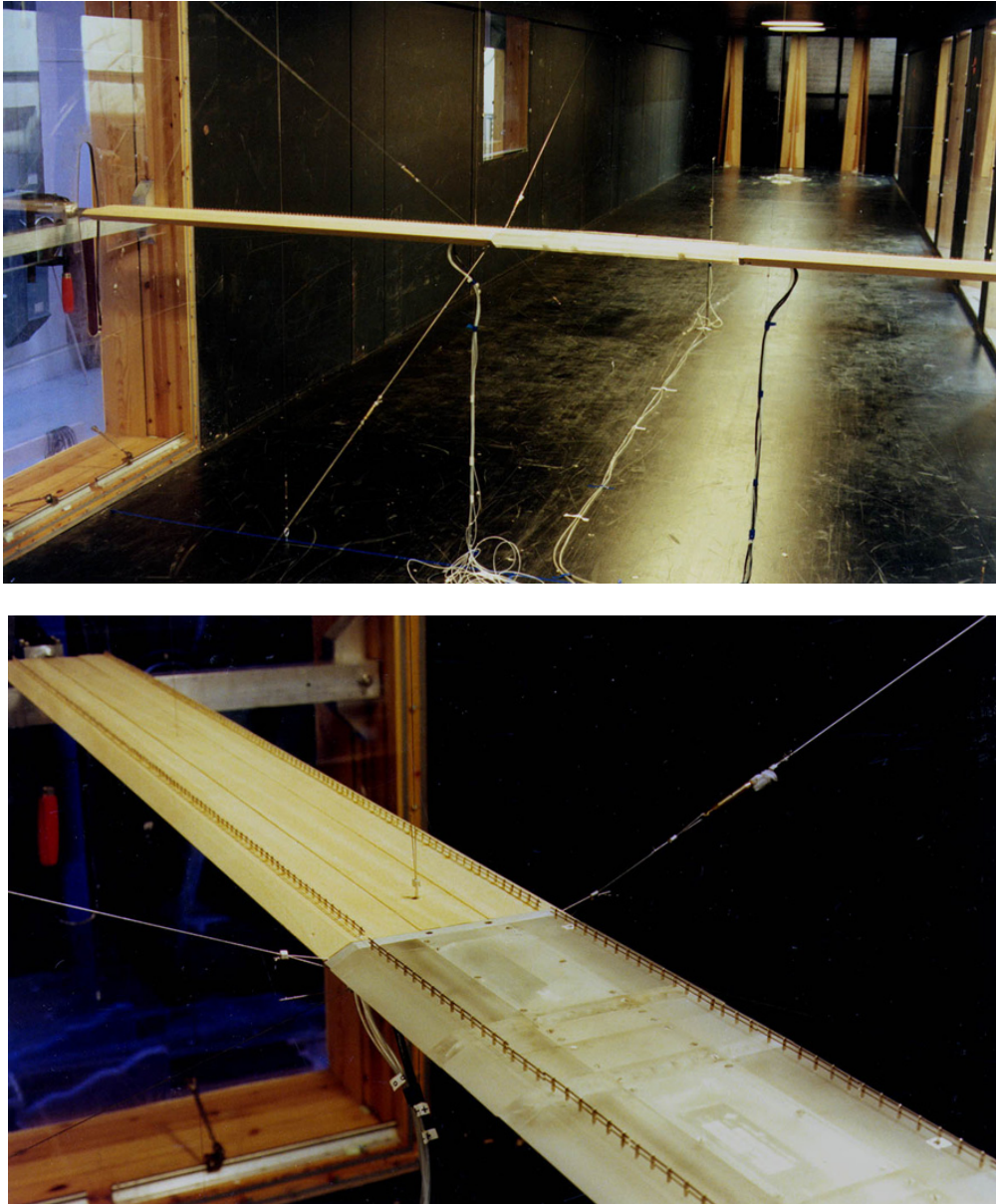
Figure 48: Views of the B/D=5 section model in DMT's Wind Tunnel II.
