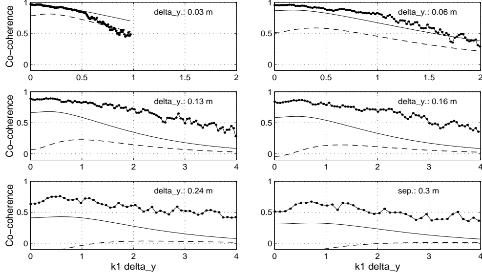
Figure 28: Co-coherence as a function of k_1 \Delta y for the lift forces (dotted line) for B/D = 12.67 and for the wind for the grid exposure . Solid line: v with L_{coh} = 0.18 and \mathcal{L} = 0.085 m; dashed line: w with L_{coh} = 0.12 and \mathcal{L} = 0.09 m.
