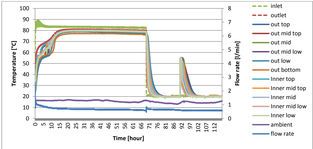
Figure 1. Temperature development and flow rate.
