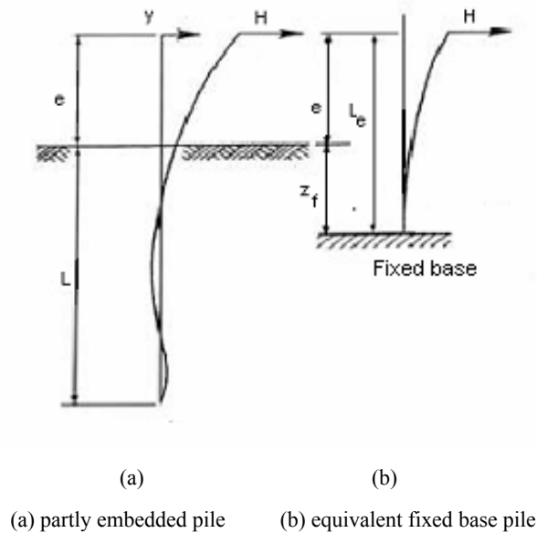
Figure 2.6 Bending of the pile
