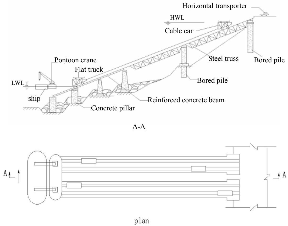
Fig. 5.3 Slope structure
