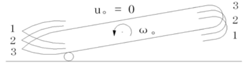
Figure 4.12. Impact on a fender of a ship with a simple rotation
