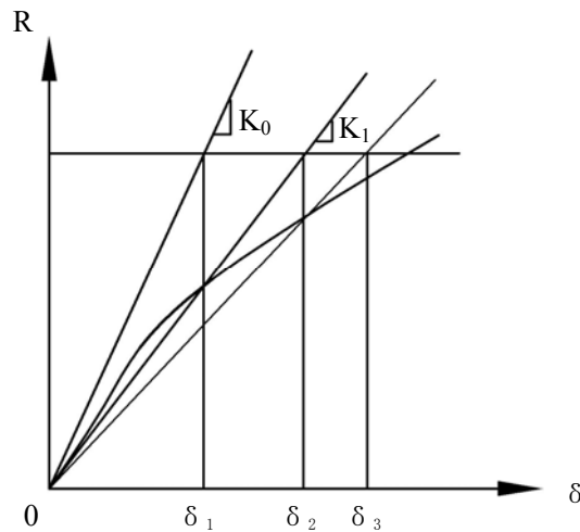
Fig.3.3 Secant stiffness method
