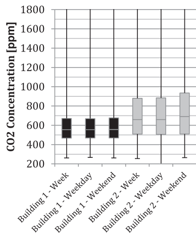
Fig. 3. Boxplot representing the median, 25th percentile, 75th percentile and min/max measurements of the CO 2 concentration [ppm] from March 2013 through April 2013.
