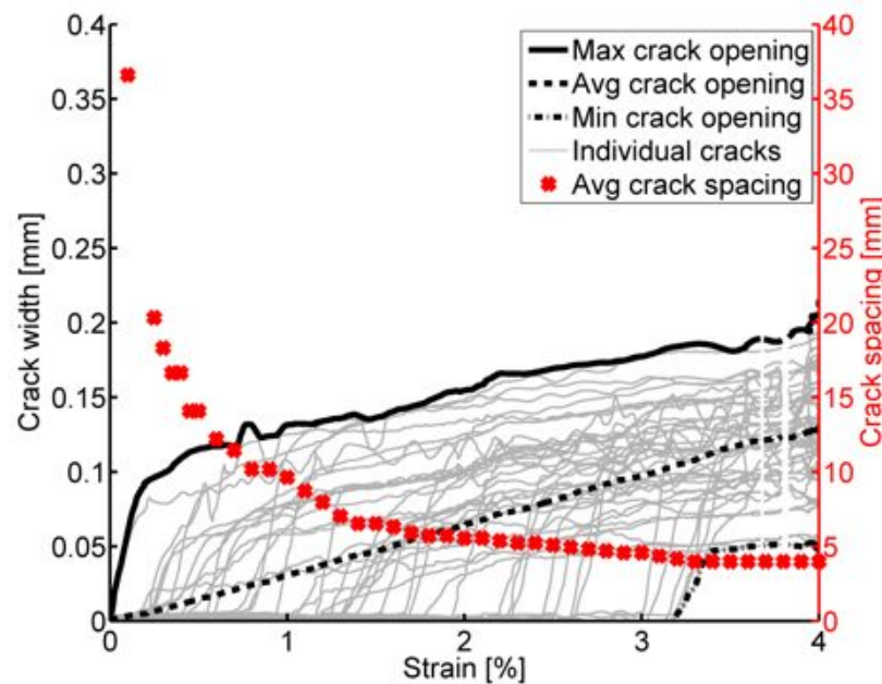
Figure 4-3 a) Stress-strain responses of three dogbone-shaped ECC tensile specimens in direct tension. b) Development of crack opening and crack spacing as a function of tensile strain obtained with DIC.
