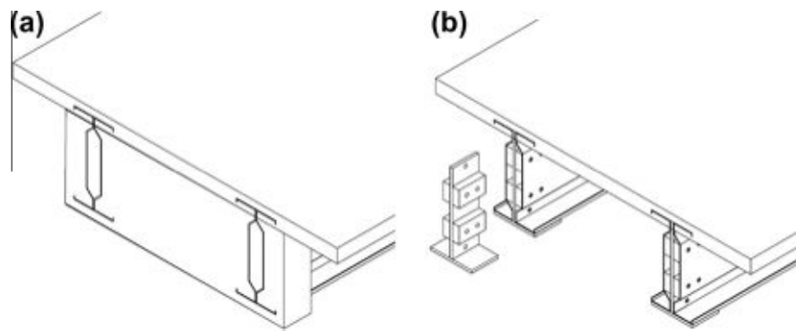
Fig. 8. A visual comparison of (a) Integrally Cast Panel 1 (ICP1) and (b) Integrally Cast Panel 2 (ICP2).
