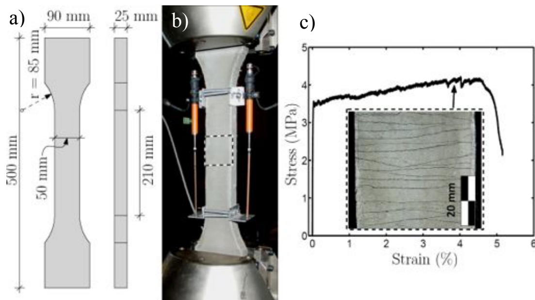
Figure 2-5 a): Geometry of an ECC dog-bone shaped specimen, b): direct tension test setup including supports and LVDT's, and c): example of tensile stress-strain response of an ECC specimens and the resulting crack pattern at approximately 4% strain.
