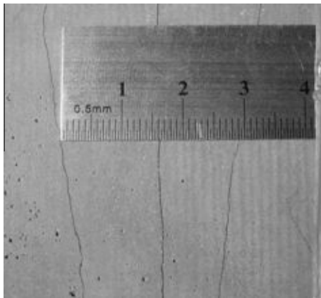
Fig. 21. Example of resulting cracks after ULS loading, figure shows multiple flexural cracks on bottom of ECC deck at mid-span.
