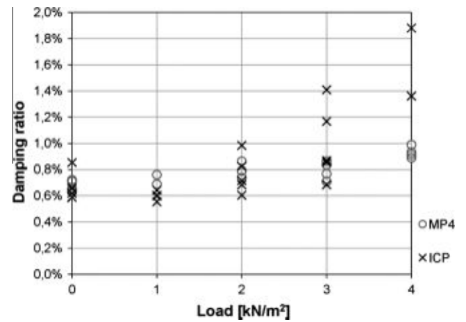
Fig. 15. Measured damping ratios for specimens MP4 and ICP as a function of additional live load.
